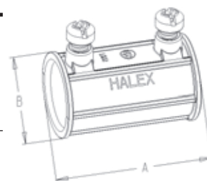
• Image shown is for 1/2" - 2". 2 1/2" - 4" has four screws.
