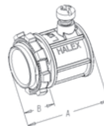
• Image shown is for 1/2" - 2". 2 1/2" - 4" has two screws.
