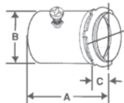
• Image shown is for 1/2" - 2". 2 1/2" - 4" has two screws.
